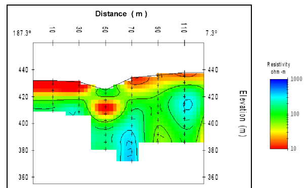
Figure 3. Line 15 Fast-Turnoff Data, Rio Tinto.
