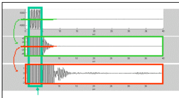
Figure 5. Monostatic radar sounding data collected in Egypt using the 3.5 MHz band of the GPR [15].
