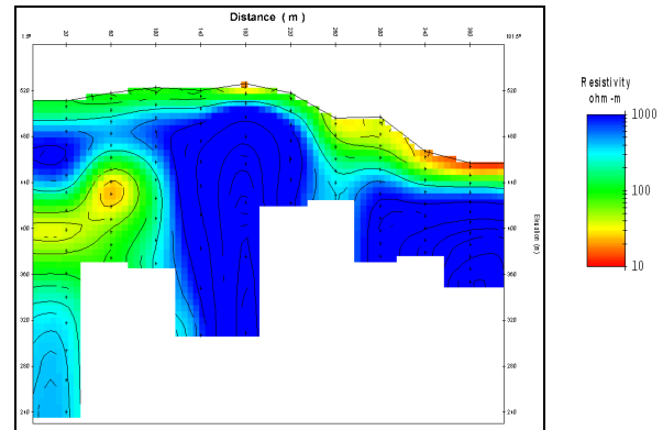
Figure 2. Line 4 Fast-Turnoff Data, Rio Tinto.
