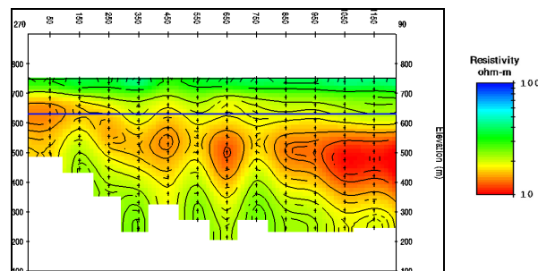
Figure 1. Line 1 TEM Data from Arizona Survey.
