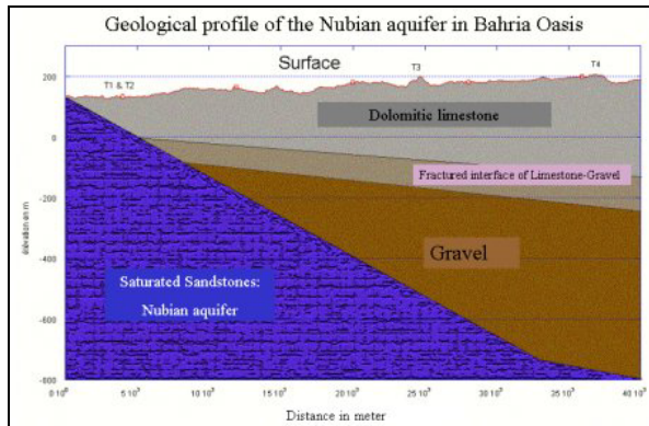
Figure 4. The hydro-geological model along the track of the GPR test experiment in the Bahria test site.
